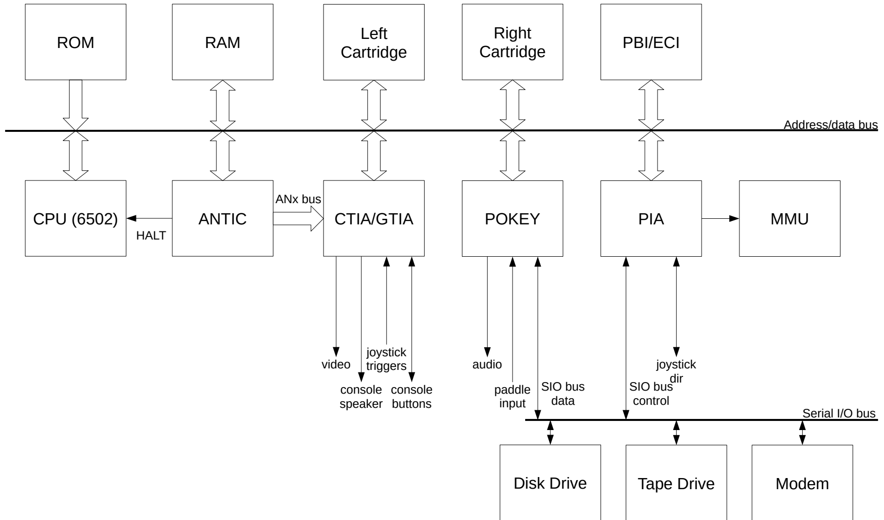
Figure 1: System Block Diagram
