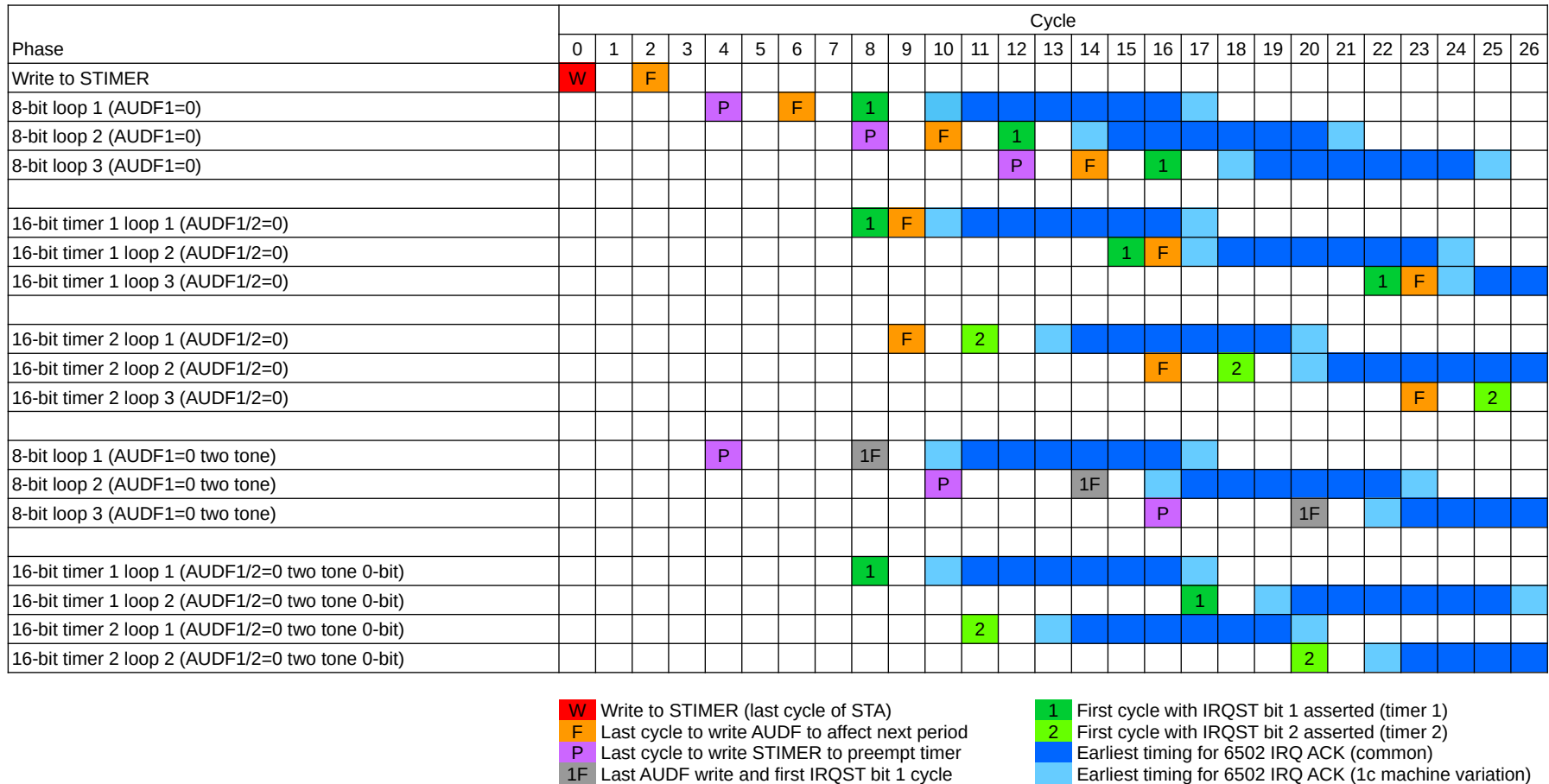
Figure 7: POKEY detailed timer timing
