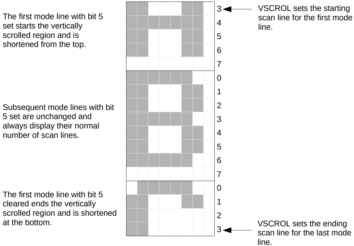
Figure 3: Effect of vertical scrolling on mode lines
