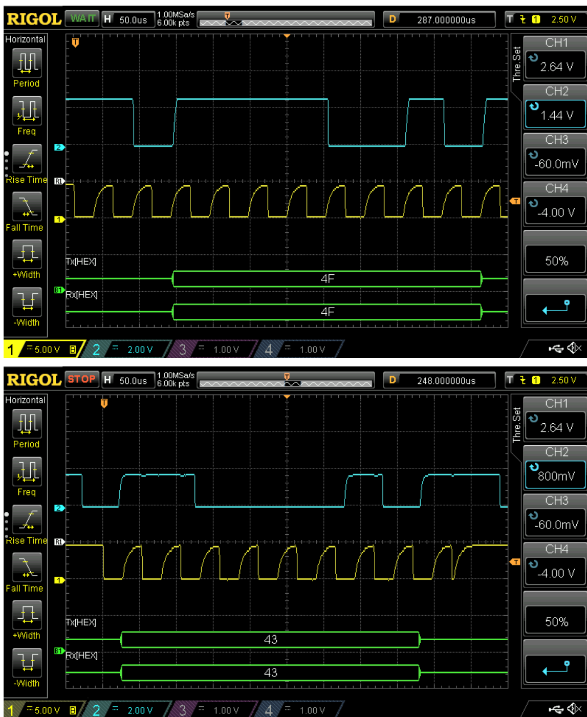
Figure 8: SIO send/receive clocking signals
