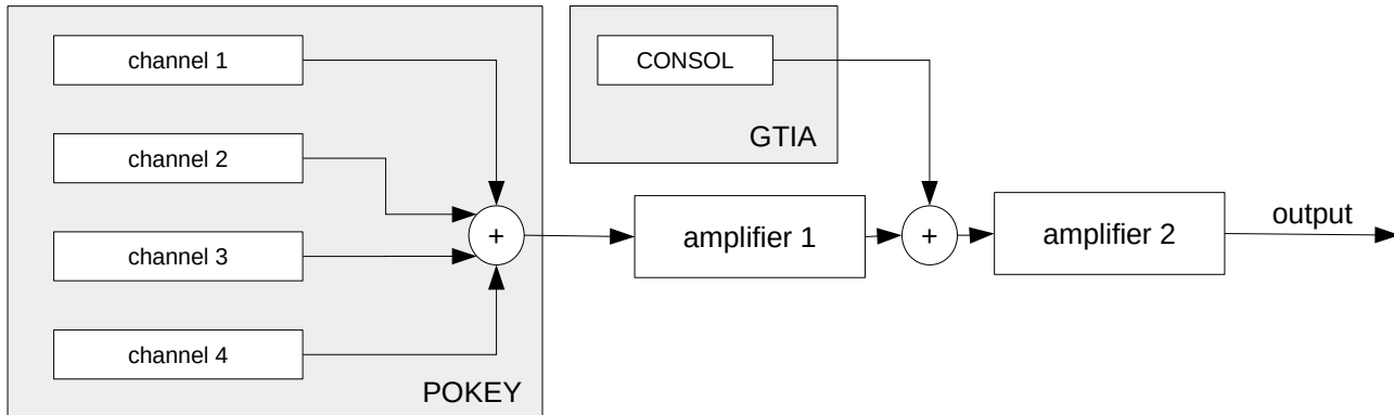
Figure 19: Analog audio block model
