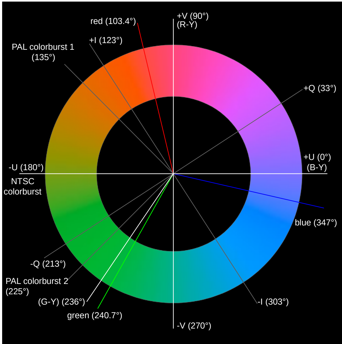
Figure 15: YIQ/YUV color space relations
