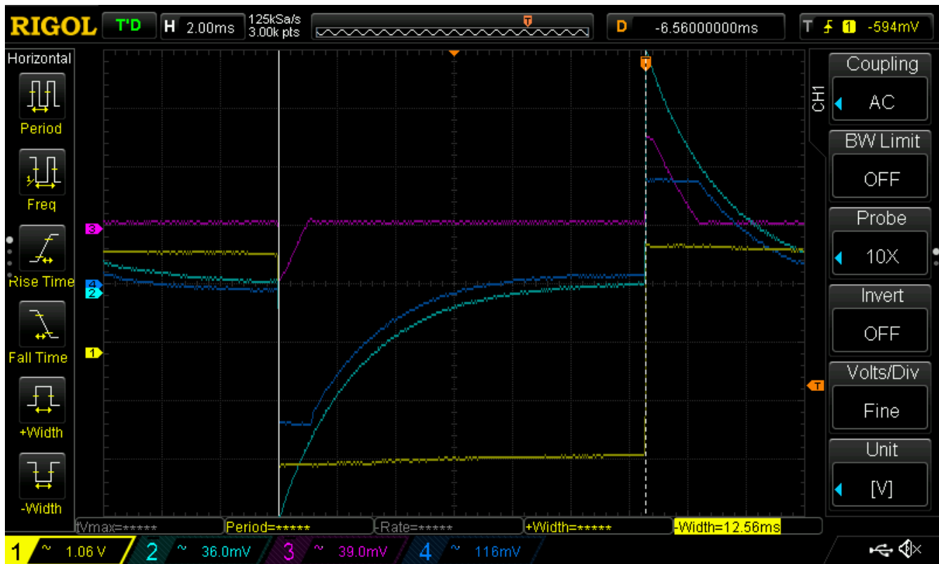
Figure 21: Dynamic clamping effect
