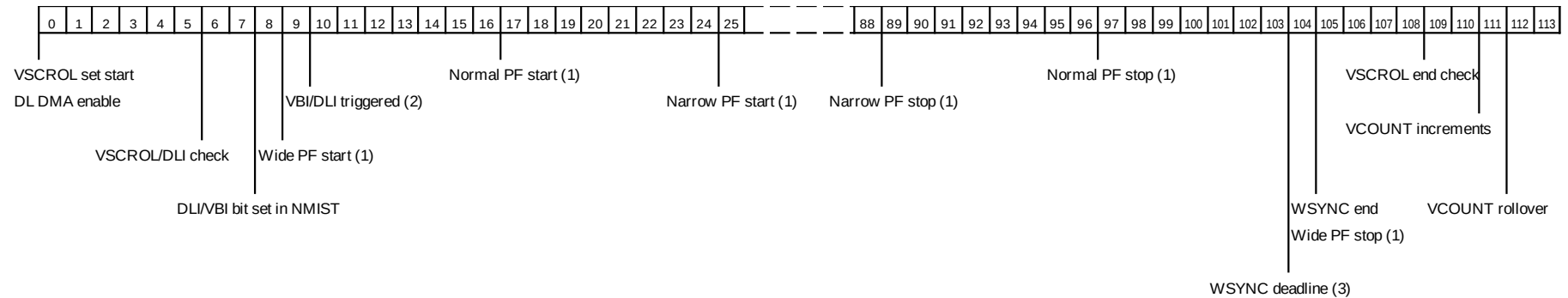
Figure 5: ANTIC event timing
