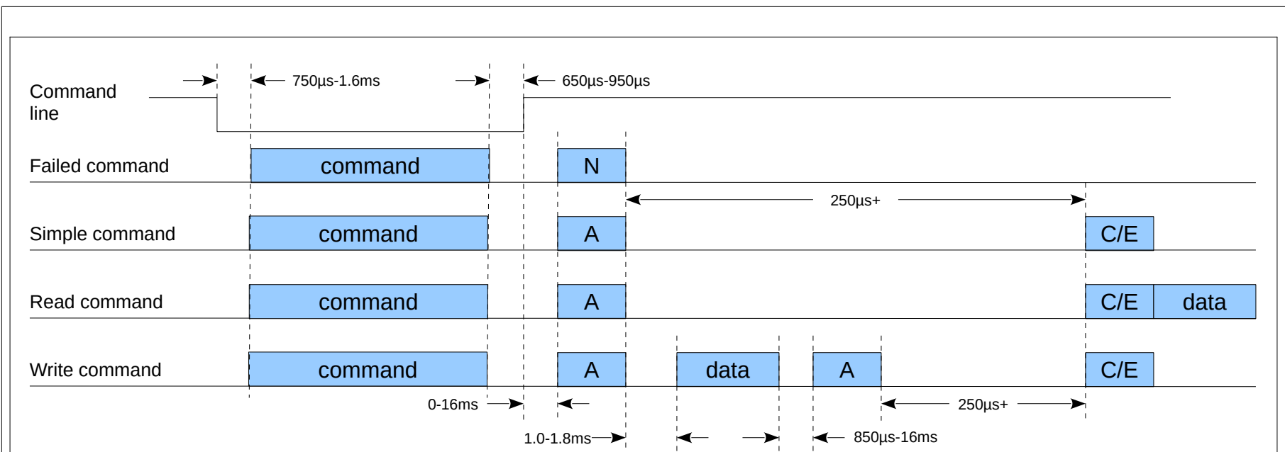
Figure 13: SIO command timing
