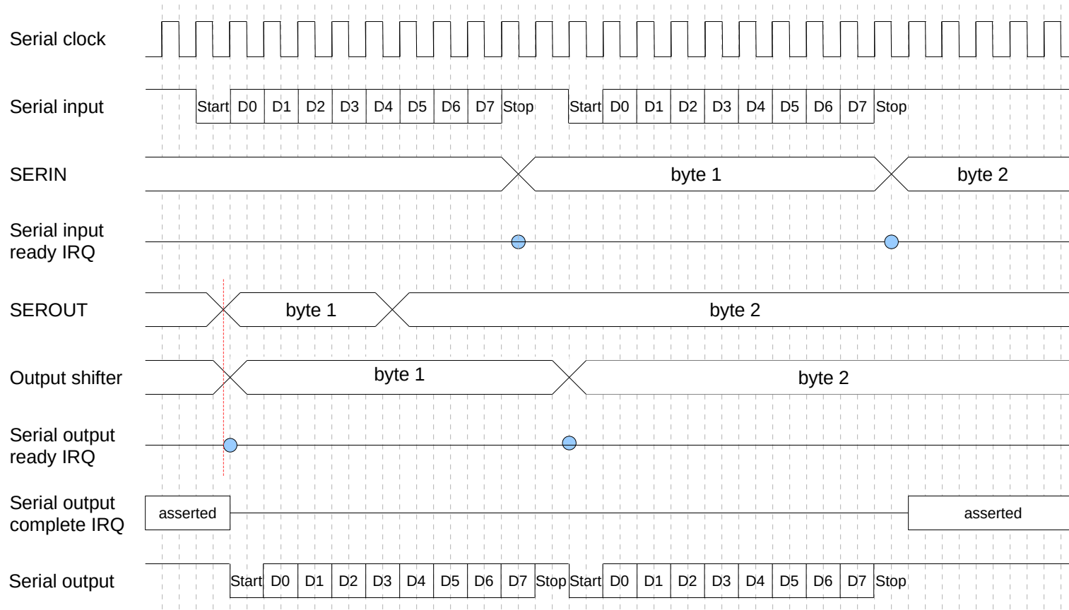
Figure 10: POKEY synchronous serial receive/transmit timing
