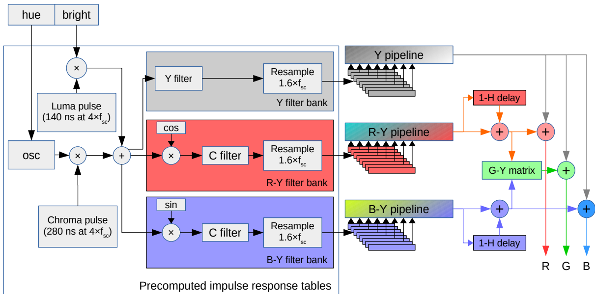
Figure 18: Altirra PAL high artifacting pipeline
