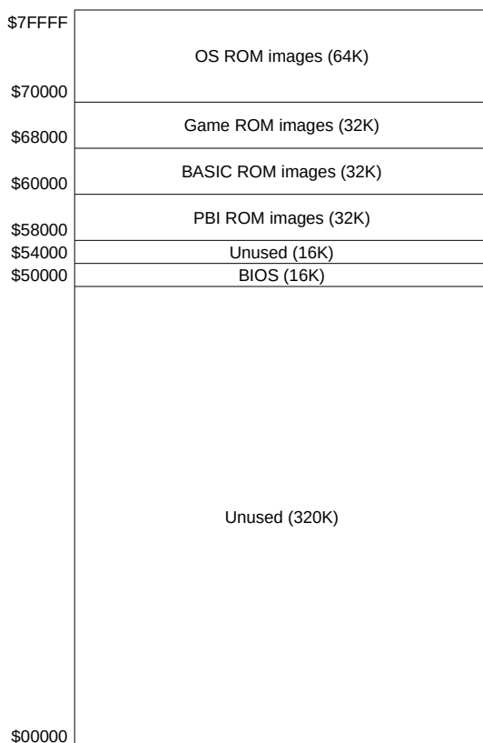
Figure 14: Ultimate1MB flash memory map
