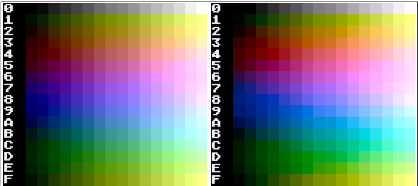
Figure 16: Effect of color correction on computed palette
