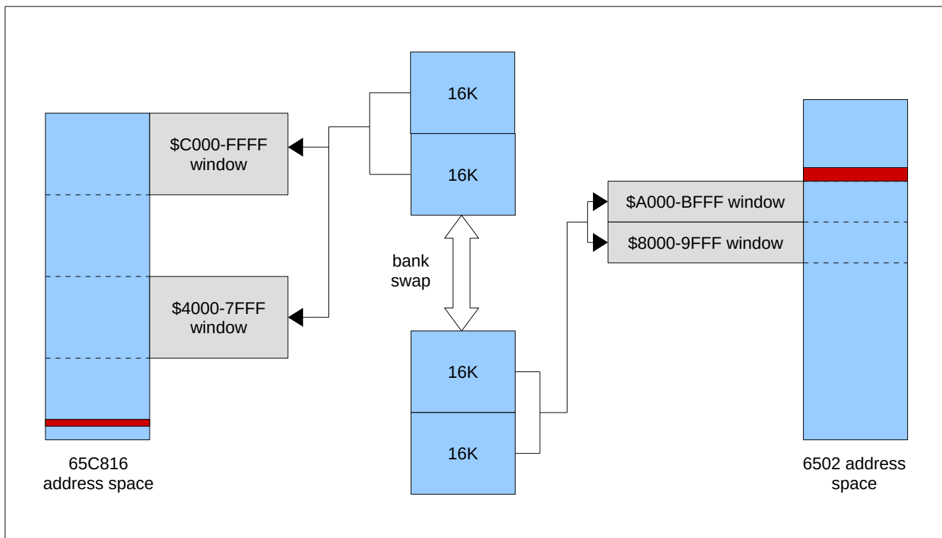
Figure 12: Veronica memory layout
